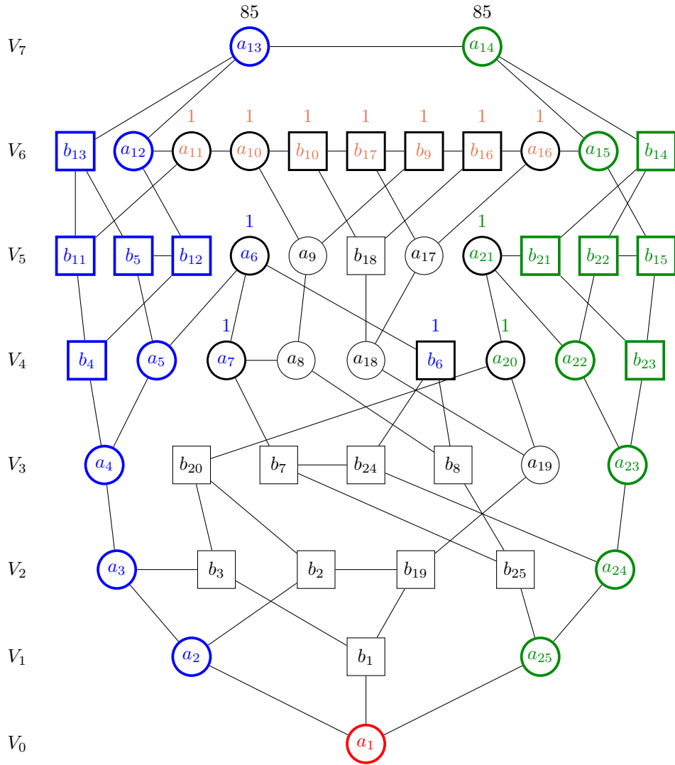
Figure 5: The Watkins graph, organized by distance from target a_1 , along with an a_1 -unsolvable configuration C of size 182.
