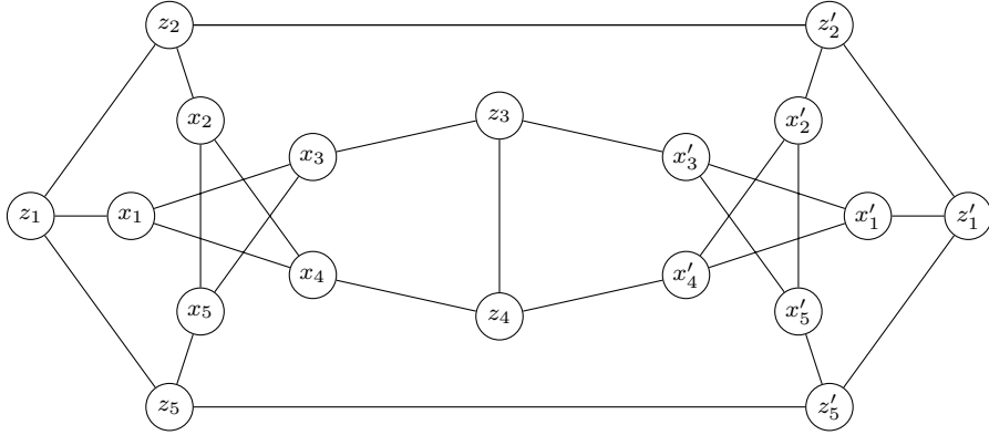
Figure 3: Blanuša 2 and its labelling.
